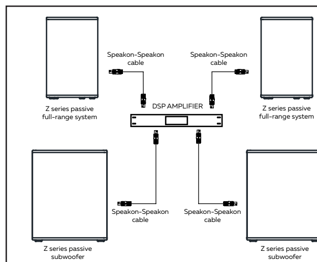
Z series passive connection diagram
